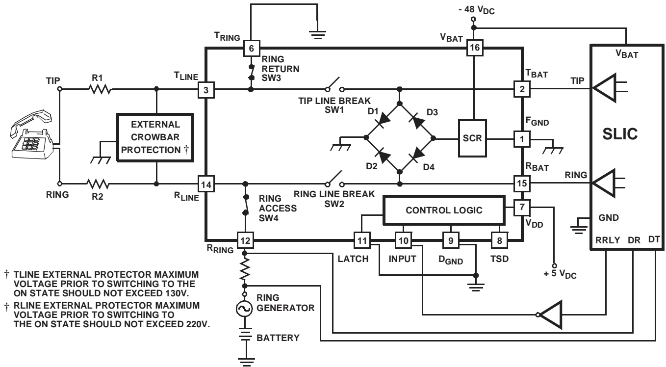
FIGURE 9. APPLICATION CIRCUIT
